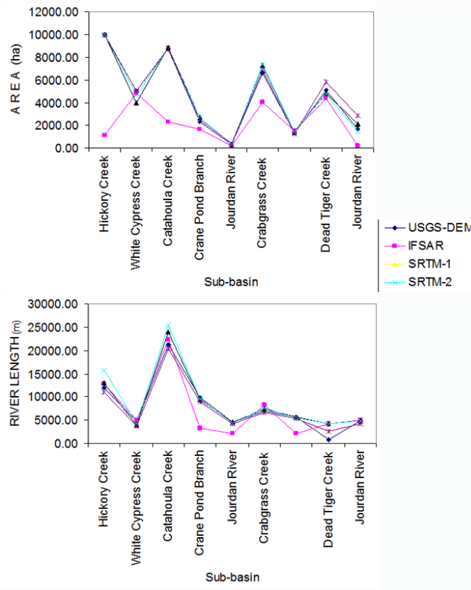
Figure 2. Topographical parameters extracted from several different topographical datasets (adapted from Alarcon & O'Hara, 2006)
