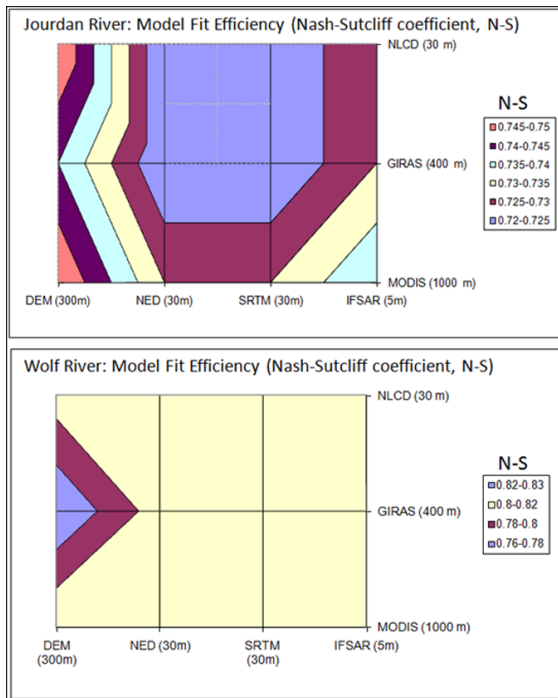
Figure 6. Final results of the land use and topography combined experiment. Notice that the combination of SRTM and MODIS provide model fit efficiencies (assessed by the Nash Sutcliff coefficient, N-S) greater than 0.725.
