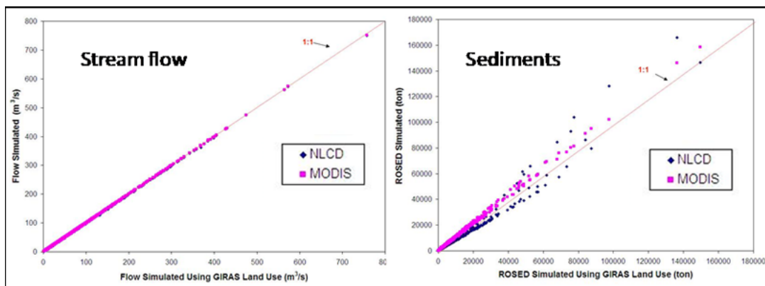
Figure 4. Scatter plot of simulated flow using GIRAS versus NLCD and MODIS (left), and total amount of sediment fraction contained in outflow simulated using GIRAS versus NLCD and MODIS (right) (adapted from Diaz et al., 2008)
